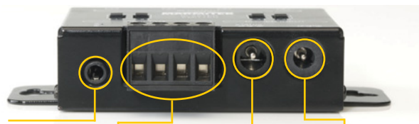
IR INPUT: Single Receiver IR INPUT: Multiple Receivers (up to 6) POWER INPUT: Status adapter POWER INPUT: Power adapter
