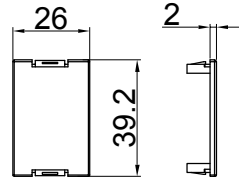
Blank module cover 2PCS
