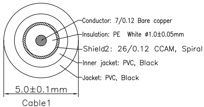
Cable construction
