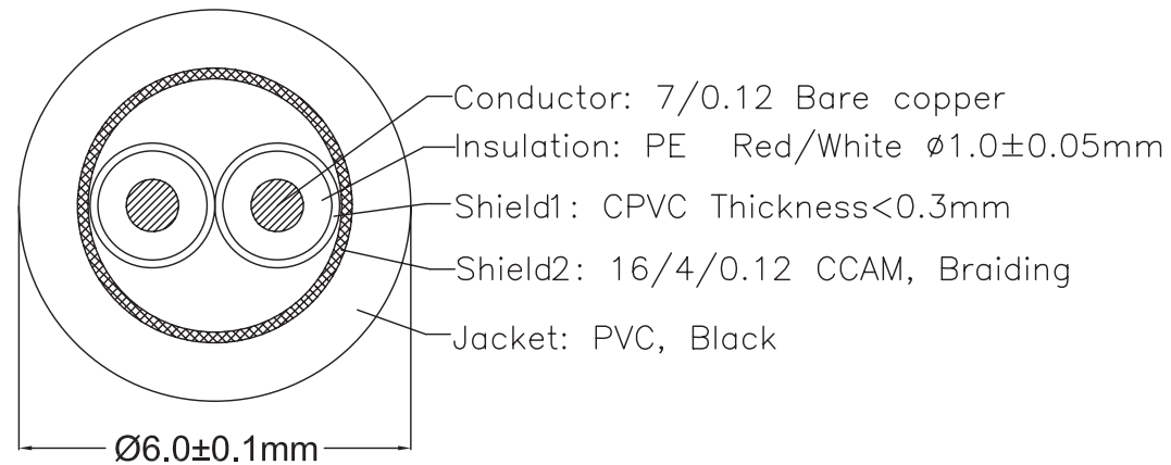
Cable Construction
