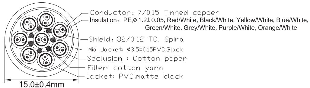
Cable Construction
