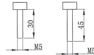
Screw M5×30 2PCS
